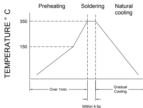
Iron Soldering times: 1 time max. Figure 2. Iron Soldering
