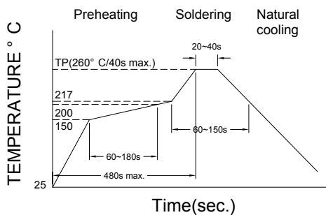
Reflow times: 3 times max. Figure 1. Re-flow Soldering
